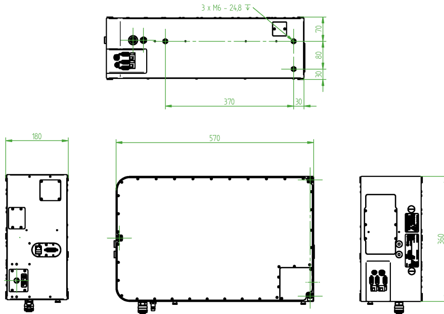
VERTICAL MOUNTING
