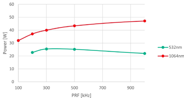
Figure 4: Power vs. repetition frequency for 1064 nm and 532 nm picosecond lasers
