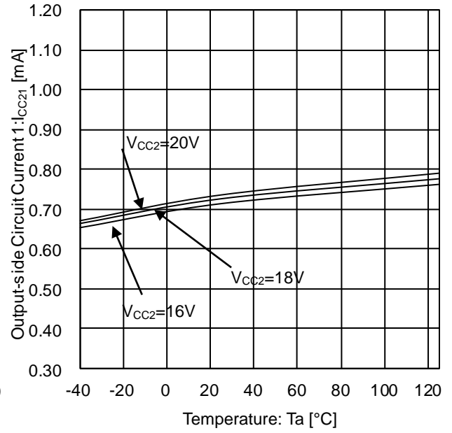
Figure 13. Output-side Circuit Current 1 vs Temperature (At OUT=L)
